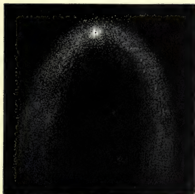
June 30.
